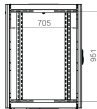
INSIDE VIEW (WITHOUT SIDE PANEL)
