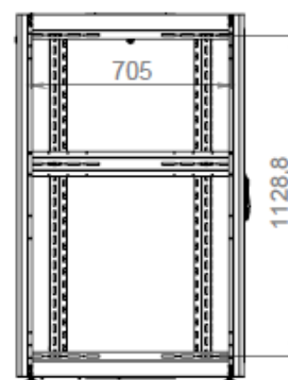
INSIDE VIEW (WITHOUT SIDE PANEL)
