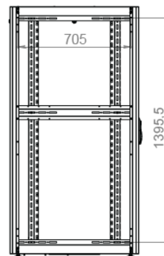
INSIDE VIEW (WITHOUT SIDE PANEL)
