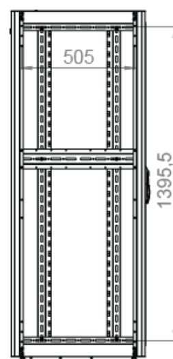
INSIDE VIEW (WITHOUT SIDE PANEL)
