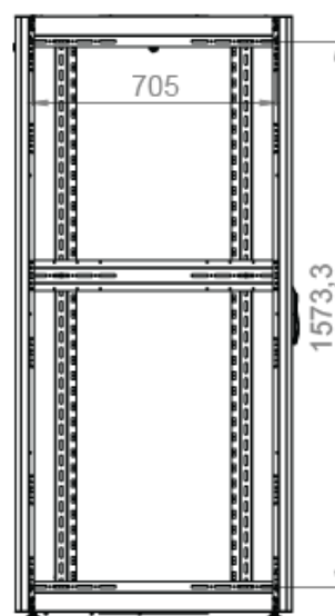
INSIDE VIEW (WITHOUT SIDE PANEL)
