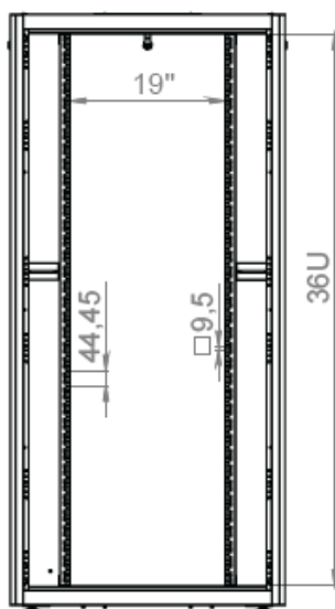
INSIDE VIEW
