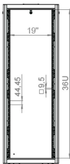
INSIDE VIEW
