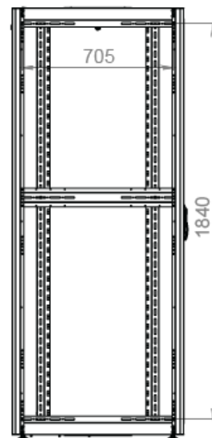
INSIDE VIEW (WITHOUT SIDE PANEL)
