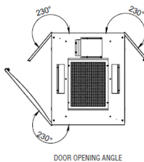
DOOR OPENING ANGLE
