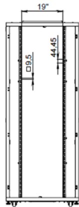
FRONT VIEW WITHOUT DOOR
