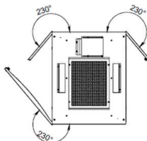
DOOR OPENING ANGLE
