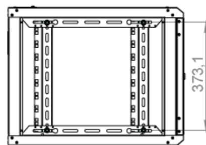
INSIDE VIEW (WITHOUT SIDE PANEL)
