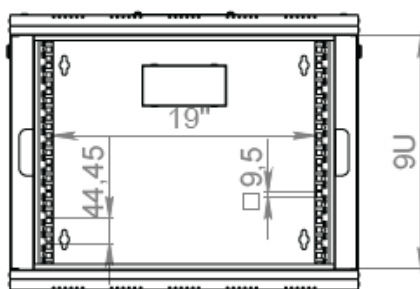
INSIDE VIEW
