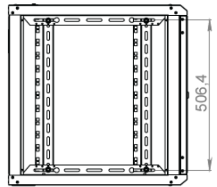
INSIDE VIEW (WITHOUT SIDE PANEL)
