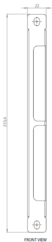
FRONT VIEW
