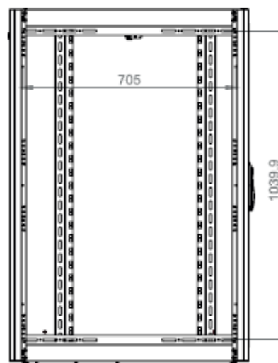
INSIDE VIEW (WITHOUT SIDE PANEL)
