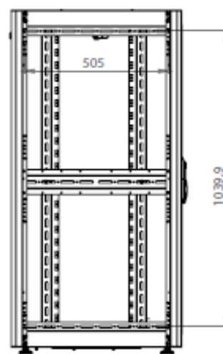
INSIDE VIEW (WITHOUT SIDE PANEL)
