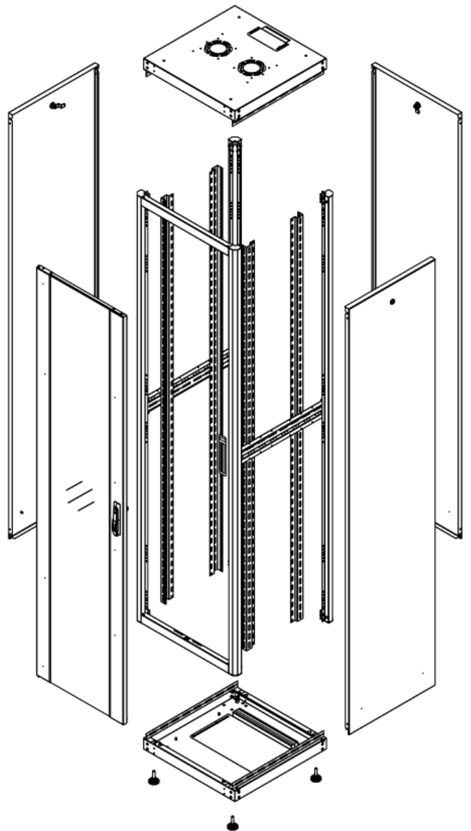
EXPLODE ISO VIEW
