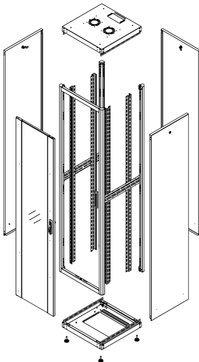
EXPLODE ISO VIEW
