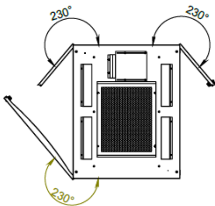
OPENING ANGLES OF DOORS
