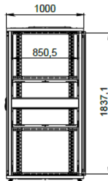
INSIDE VIEW WITHOUT SIDE PANEL
