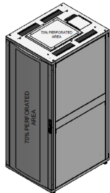
ISOMETRIC VIEW
