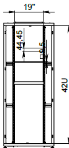
INSIDE VIEW WITHOUT DOOR
