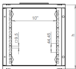
FRONT VIEW WITHOUT DOOR
