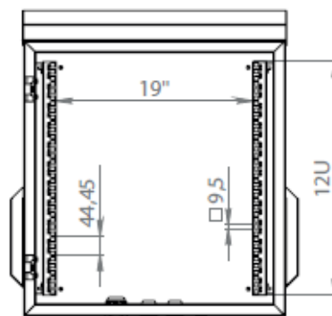
INSIDE VIEW
