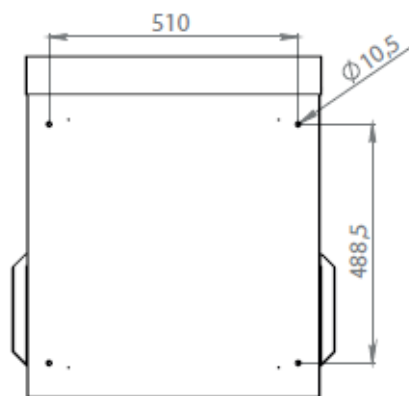
BACK VIEW
