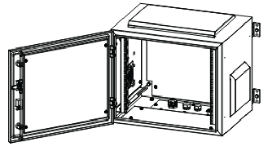
Isometric View
