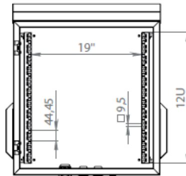
INSIDE VIEW
