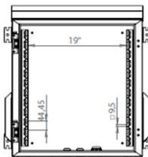
Front View Without Door
