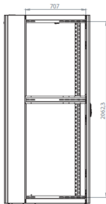
SIDE VIEW (WITHOUT SIDE PANEL)
